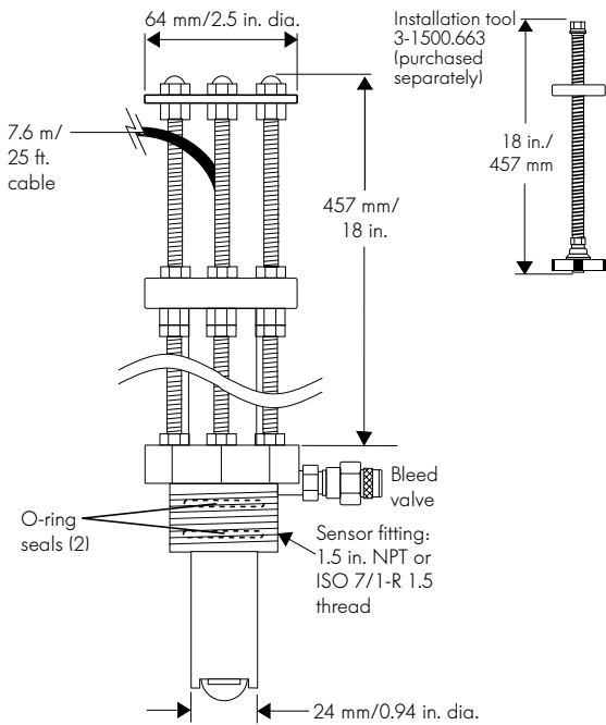
2540/2541/2517 Hot-Tap for 1.5 to 36 in. pipes
